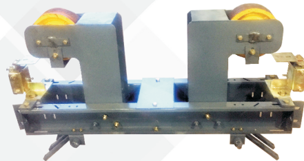
MRL Car Frame
