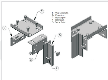
Car & Counter Brackets
