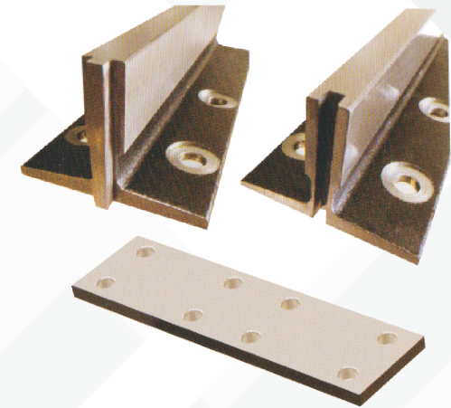
Guide Rails & Fish Plate
